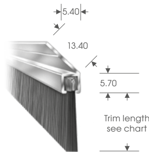
No. 1 Section - XSmall
