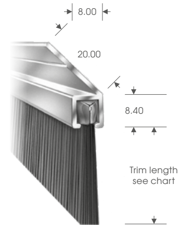
No. 3 Section - Medium
