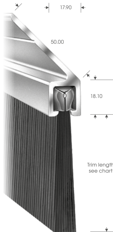
No. 6 Section - XXL Large
