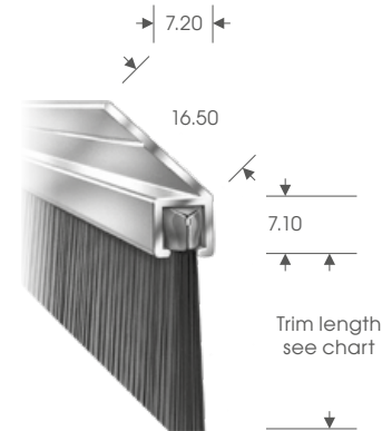
No. 2 Section - Small
