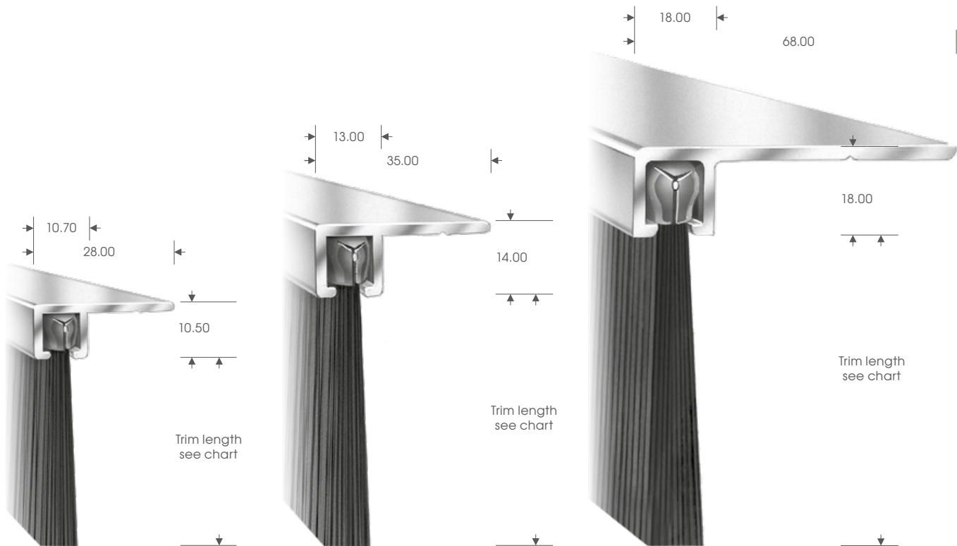
No. 4 Section - Large
