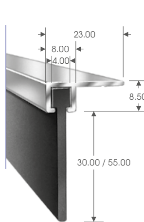
Rubber seal 90°
