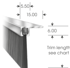
No. 1 Section - XSmall
