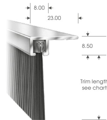
No. 3 Section - Medium
