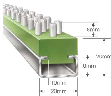
Lath brush - Ref: LB37 Lath carrier - Ref: LC37
