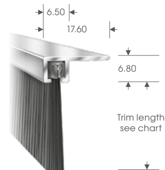
No. 2 Section - Small
