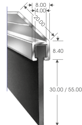
Rubber seal 45°
