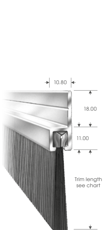
No. 4 Section - Large
