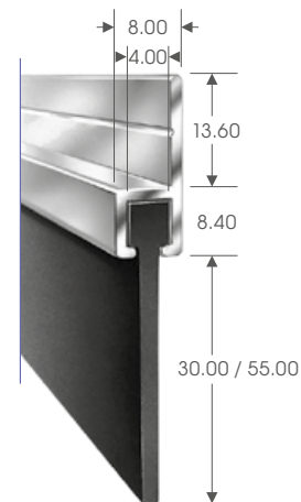
Rubber seal 180°
