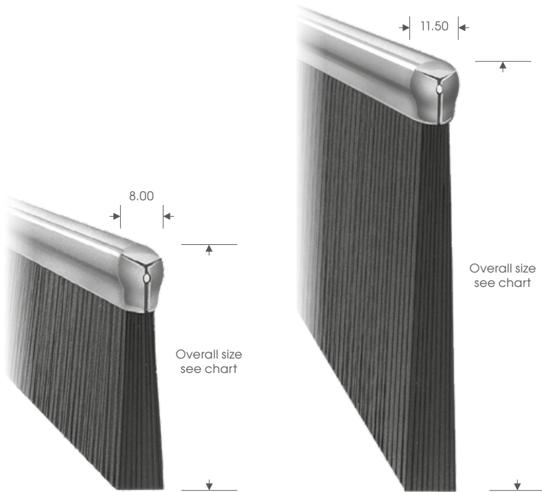
No. 5 Section - XLarge
