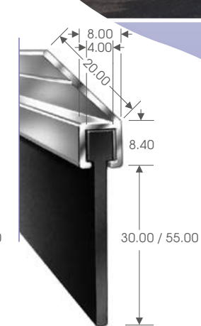
Rubber seal 45°
