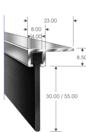
Rubber seal 90°
