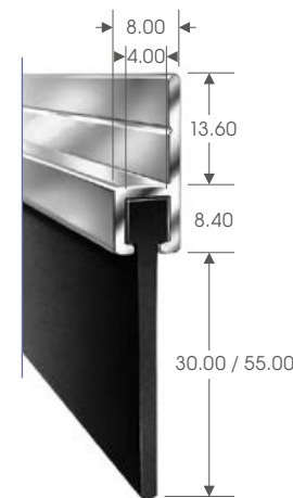
Rubber seal 180°
