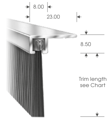
No. 3 Section - Medium
