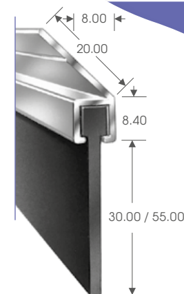
Rubber Seal 45°
