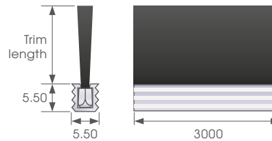
Ref: Rebate 1
