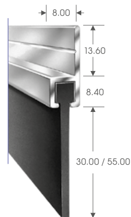
Rubber Seal 180°
